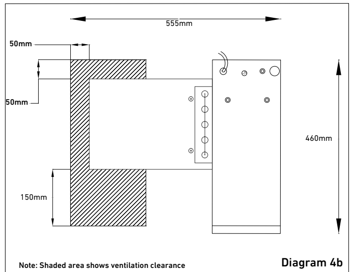
Quadra Sparkling Suggested Layout B (Plan)
