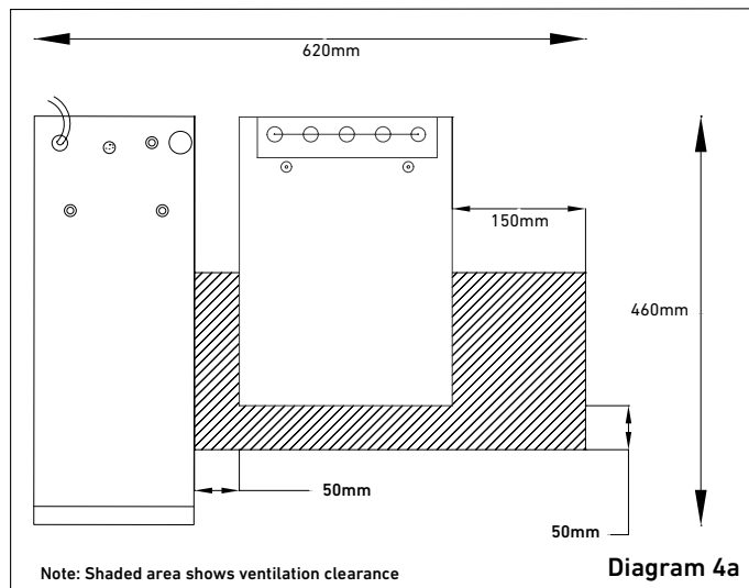
Quadra Sparkling Suggested Layout A (Plan)
