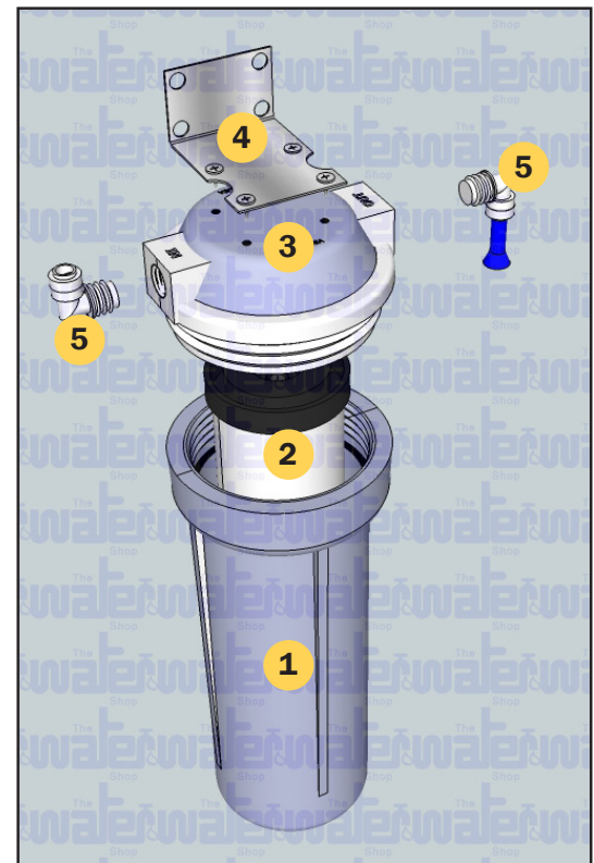
Diagram 3 - Labelled Assembly of Components
